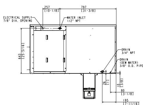
AIR-COOLED
