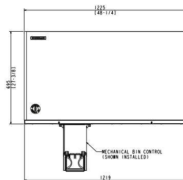
REMOTE AIR-COOLED
