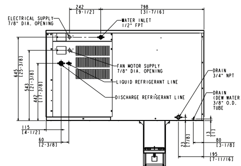
REMOTE AIR-COOLED
