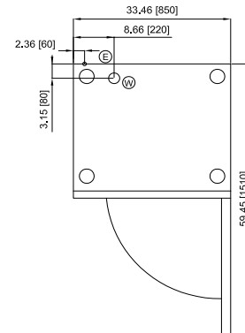
PLAN VIEW
