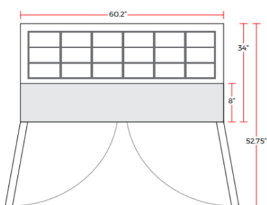
SP60 TOP VIEW
