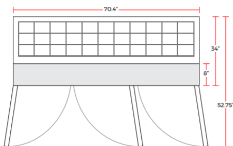
SP72 TOP VIEW
