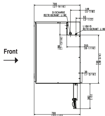
REMOTE AIR-COOLED
