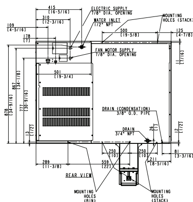
REMOTE AIR-COOLED
