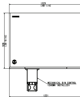
REMOTE AIR-COOLED
