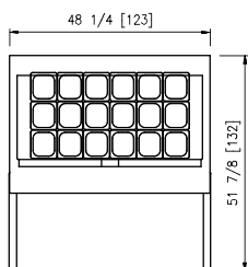
TOP NLSMP48-18
