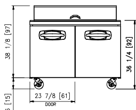
FRONT NLSMP48-18
