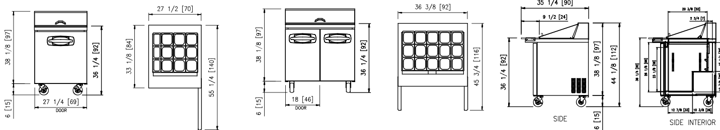
FRONT NLSMP27-12
