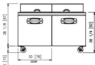
FRONT NLSMP60-24
