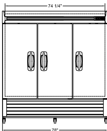
NLR72-S FRONT
