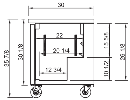
SIDE INTERIOR
