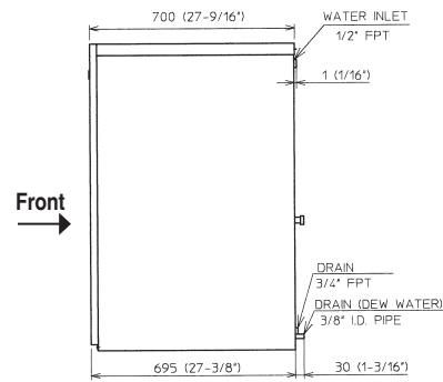
REMOTE AIR-COOLED
